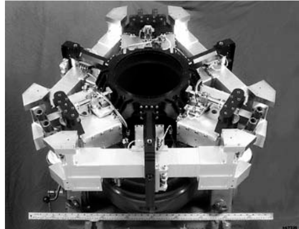
Figure 7. Secondary mirror tilt mechanism at Lockheed, August 1997.
